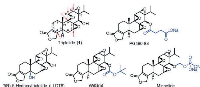
Figure 1. Structures of triptolide and triptolide analogues under clinical development. Potential sites of attack by a nucleophile from a protein are marked with red arrows. Sections for which the analogues differ in structure from triptolide are highlighted in blue.
